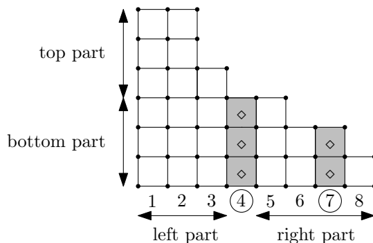
FIGURE 4. An example of a Ferrers diagram with two \diamond -columns. The left, right, top, and bottom parts are shown.
