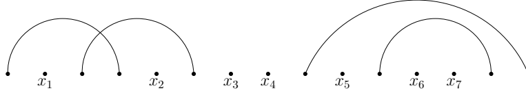
FIGURE 11. A prefix of a matching with seven stubs, forming four equivalence classes \{x_1, x_2\} , \{x_3\} , \{x_4\} , and \{x_5, x_6, x_7\} .
